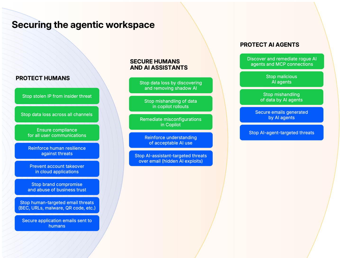
Figure 3: Securing the agentic workspace means deploying layered collaboration and data security capabilities to protect humans, AI assistants and AI agents.
